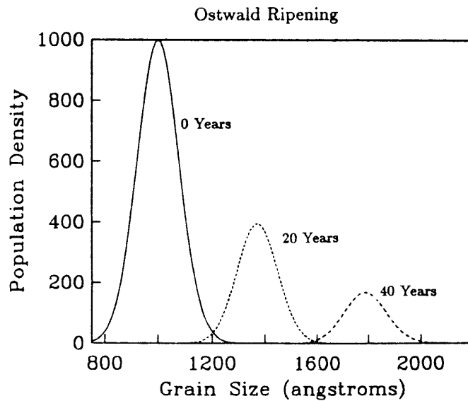
Figure 3-10: Effect of Ostwald ripening on the quantity and size of an initially Gaussian population of gibbsite crystals with an average size of 1000Å, using an interfacial energy of 350 mJ/m 2 . From Steefel and Van Cappellen (1990).
