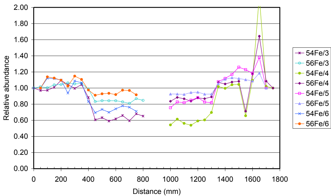
Figure 6-21: Profile of various isotopes of Fe across the interface of sample A2.
