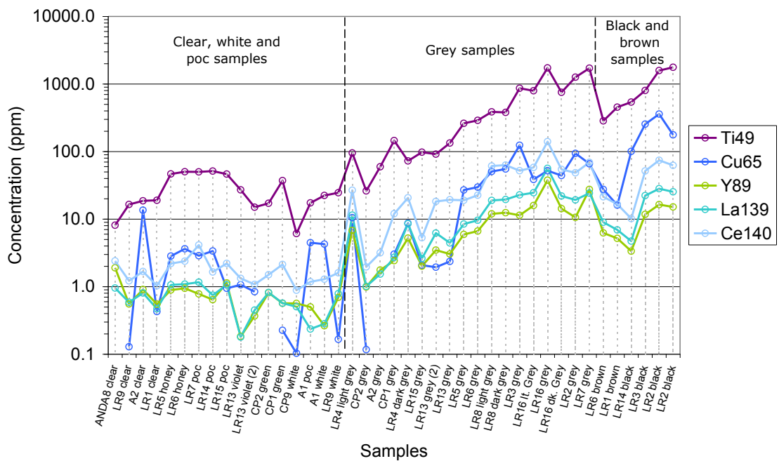
Figure 5-11: Elemental abundance of Ti, Cu, Y, La and Ce for all bands within the samples investigated.
