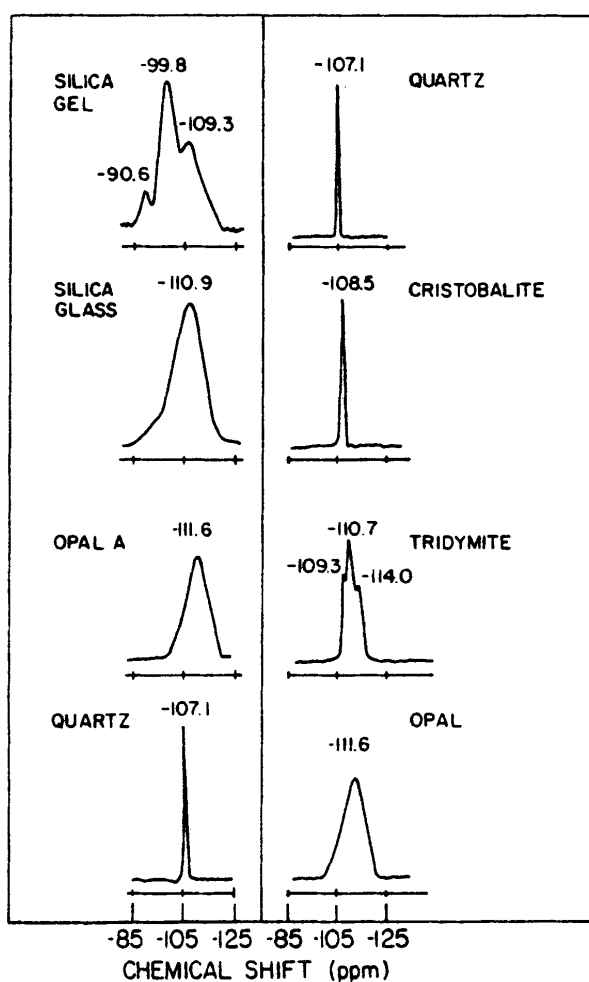
Figure 7-3: NMR spectra of various \text{SiO}_2 polymorphs. From de Jong et al. (1987).
