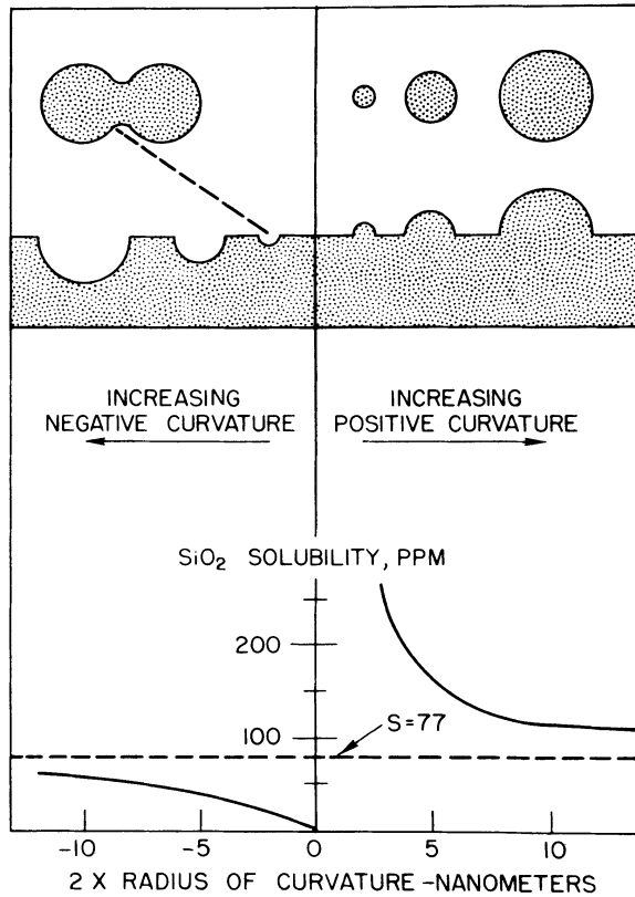
Figure 3-9: SiO 2 solubility vs. radius of curvature. From Iler (1979).
