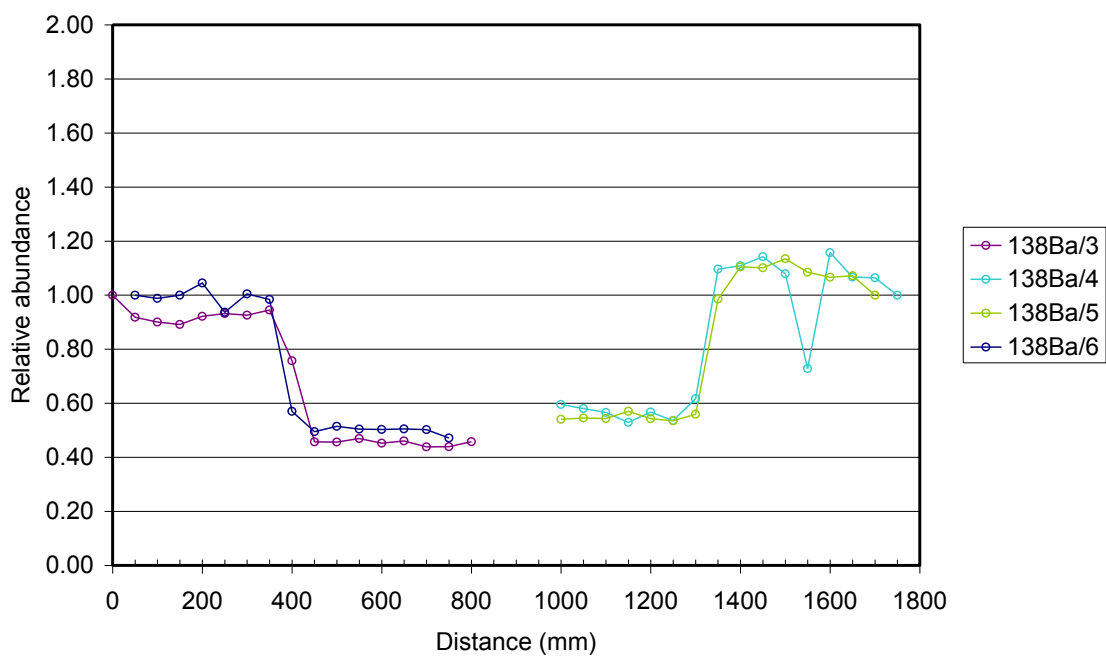
Figure 6-19: Trend of Ba across the interface of sample A2.
