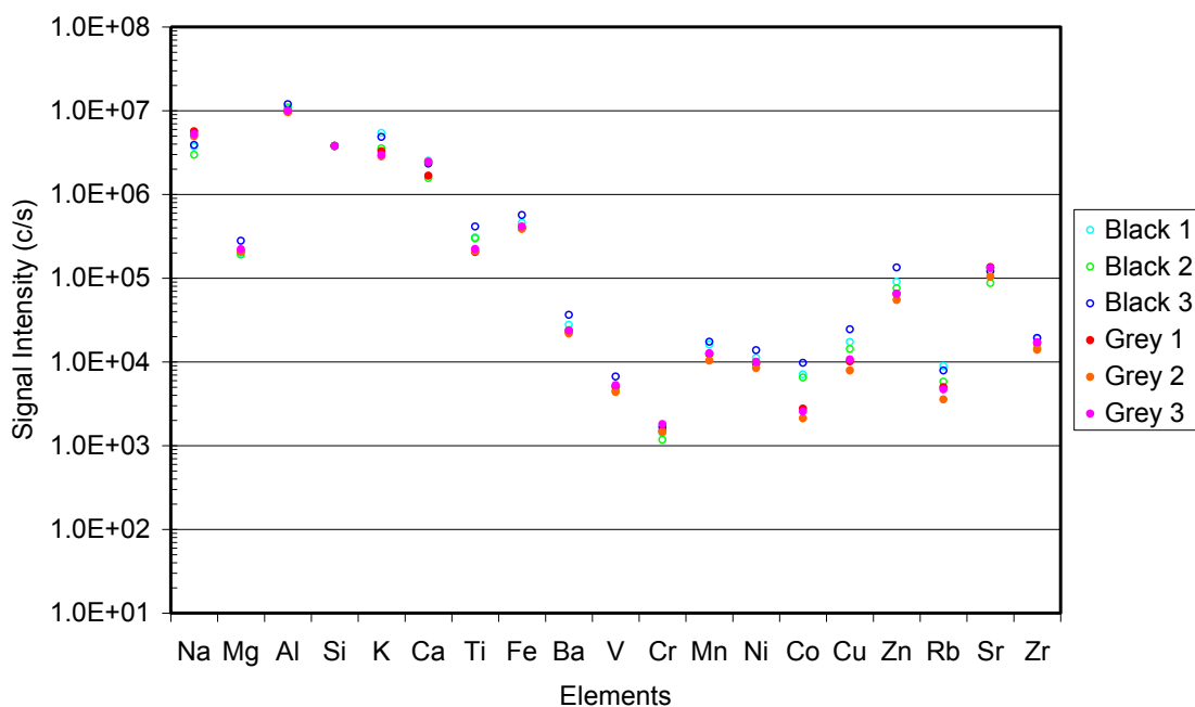
Figure 6-11: Graphical representation of the abundance of elements at each spot in sample LR3.
