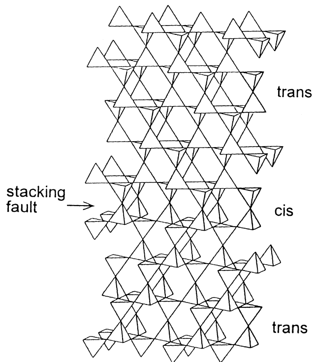
Figure 2-9: Tridymite stacking fault (cis) in a cristobalite sequence (trans). Each tetrahedron represents one SiO 4 group. From Graetsch et al. (1994).
