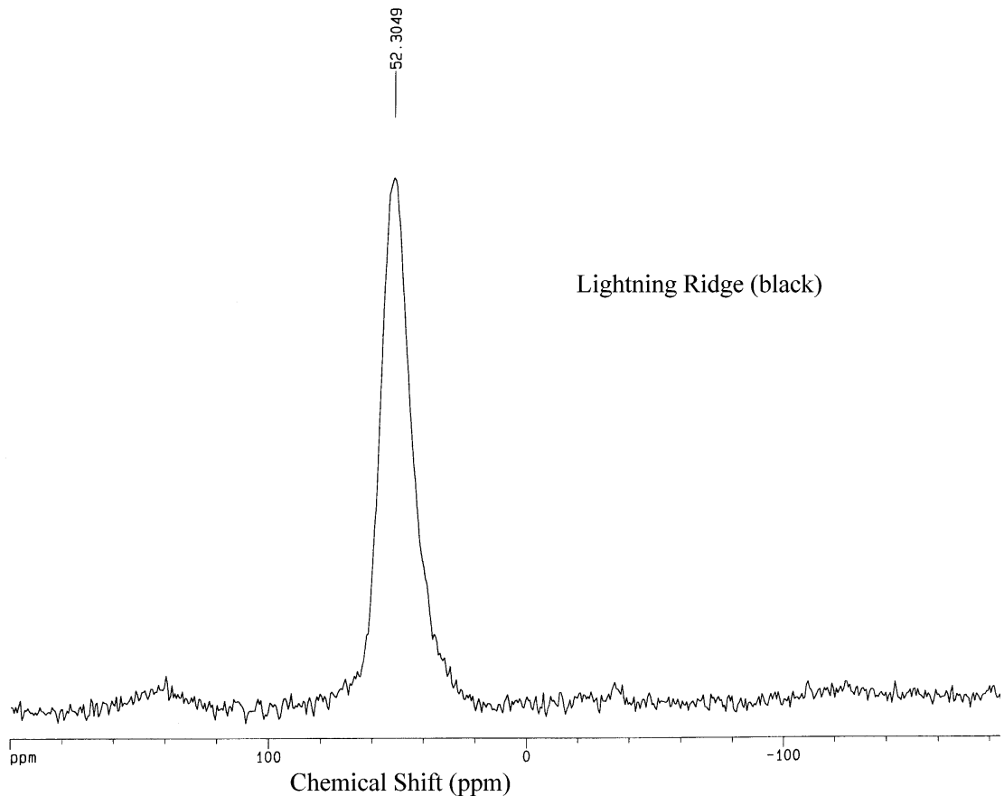
Figure 7-17: 27 Al NMR of opal-AG from Lightning Ridge. The small peak at 140 ppm is a spinning sideband.
